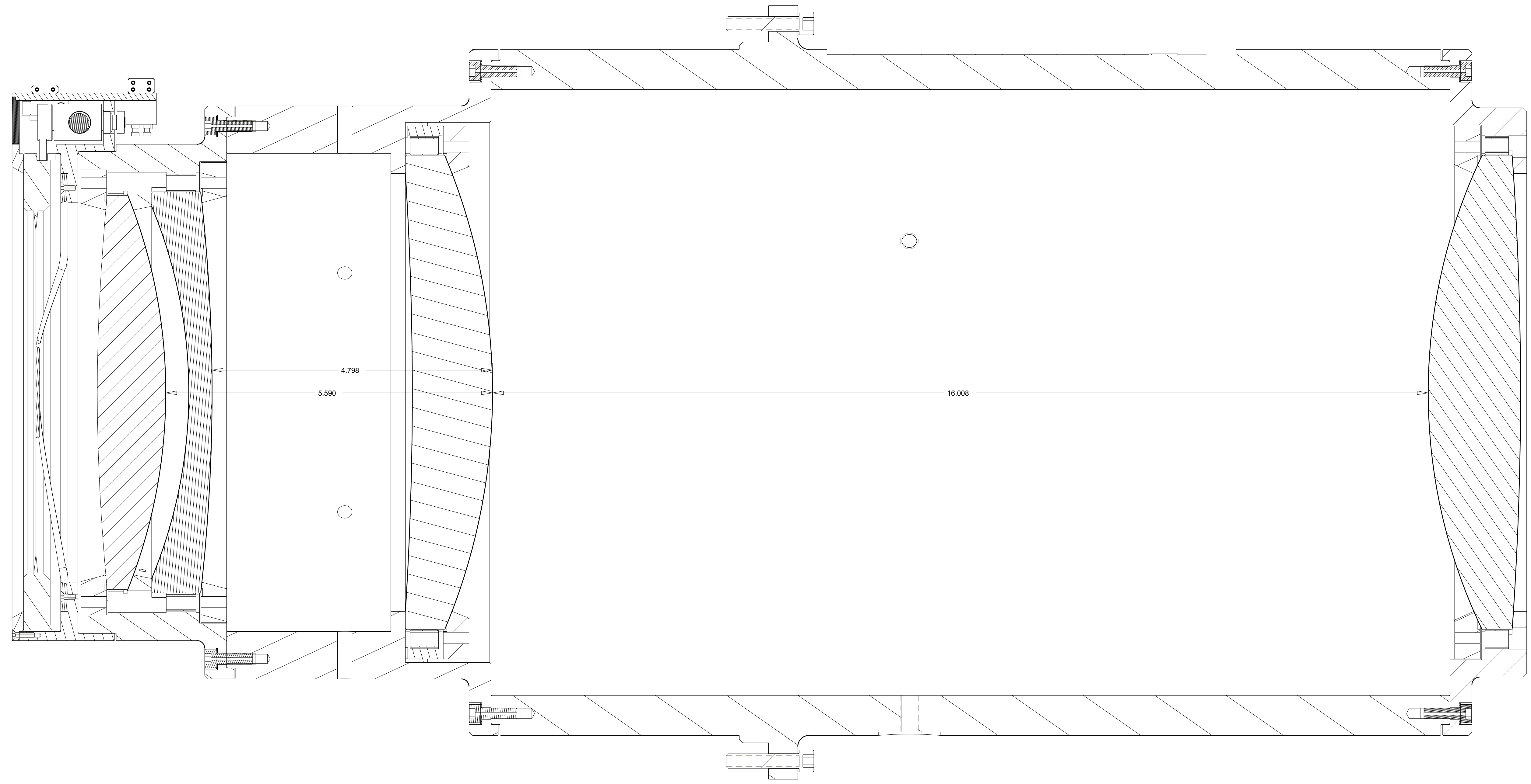
SECTION C-C SCALE 1 : 1
