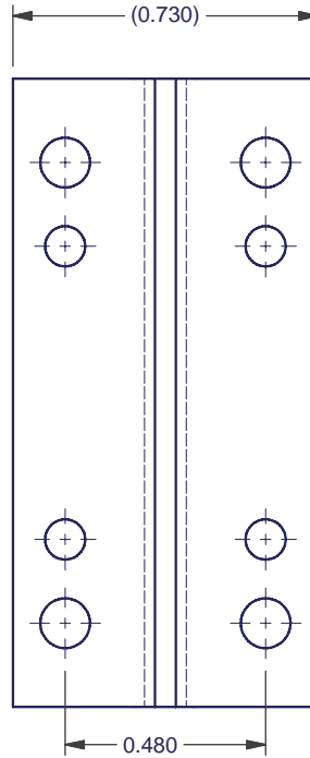
FOLDED PART SCALE 2 : 1
