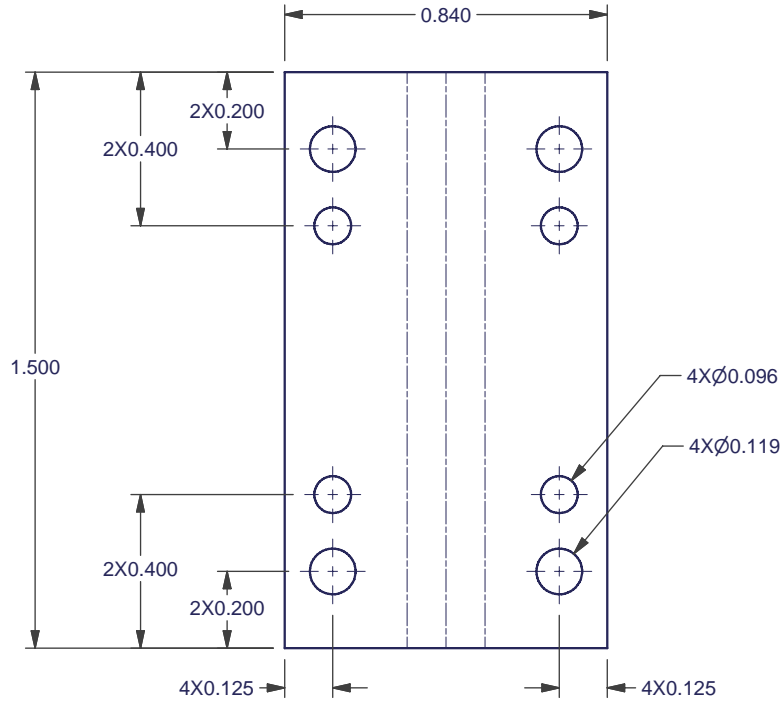
FLAT PATTERN SCALE 2 : 1
