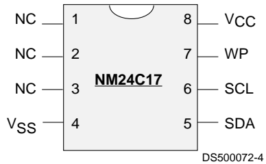
Dual-In-Line Package (N), 8-Pin SO Package (M8) and 8-Pin TSSOP Package (MT8)
