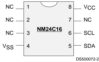
Dual-In-Line Package (N), 8-Pin SO Package (M8) and 8-Pin TSSOP Package (MT8)
