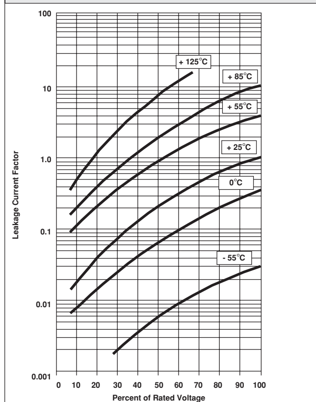
TYPICAL LEAKAGE CURRENT FACTOR RANGE
