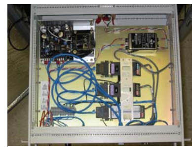
RS-422 & PRESSURE TRANSDUCER EXCITATION
