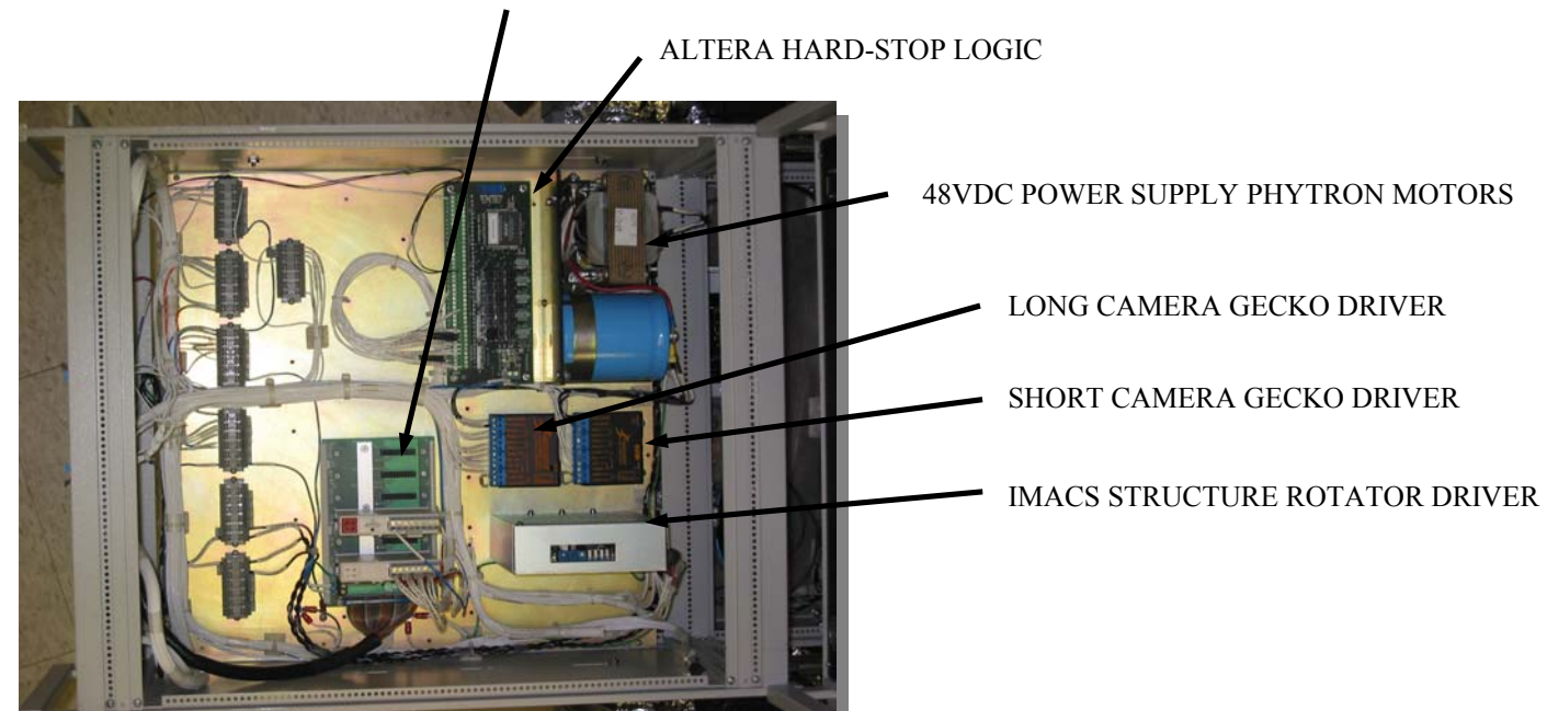
DIGITAL I/O MR4A
