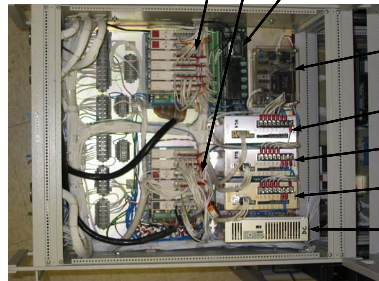
ALTERA HARD-STOP LOGIC
