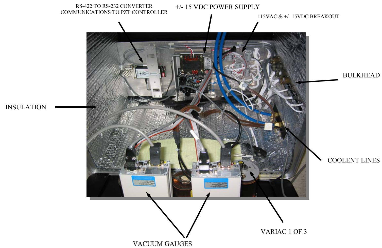
BLACK ABS BOX INSIDE INSTRUMENT
